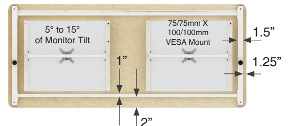
Underside View
